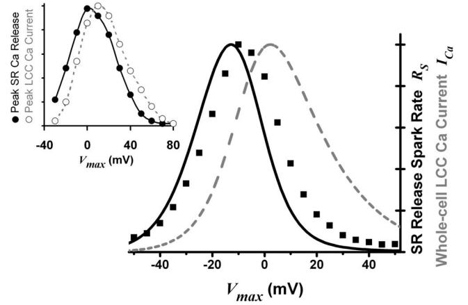
FIG. 4. Analytical (solid line) and numerically simulated (■) spark rate R_S as a function of V_{max} ( g=0.910 \mu\text{m}^3\text{s}^{-1} ); whole-cell I_{Ca} (dashed line). Inset: Experimental values from [4] for peak SR release current (●) and peak LCC current (○). (All plots normalized to peak height.)
