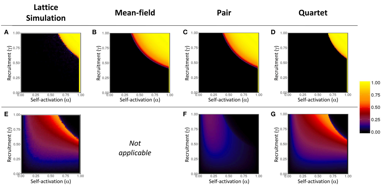
FIGURE 10 | Heatmap visualization of amplitude coefficient A (top row, A–D ), and clustering coefficient Q (bottom row, E–G ), in \alpha - \gamma parameter space. Values measured at the end of 500,000 steps, for numerical simulations and for mean-field, pair, and quartet approximations. The narrow vertical band of maximum amplitude ( A \approx 1 ) is the trivial case at \alpha = 1 wherein the entire lattice oscillates in unison. The clustering coefficient cannot be calculated for the mean-field approximation. The color scale applies to both A and Q ; rare negative values of Q were very near zero and are represented as such in the plot.
