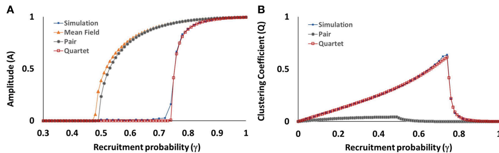
FIGURE 9 | Amplitude coefficient A ( A ) and clustering coefficient Q ( B ) as a function of recruitment probability \gamma , for self-activation probability \alpha held at 0.80. Values measured at the end of 500,000 steps, for numerical simulations and for mean-field, pair, and quartet approximations. The clustering coefficient cannot be calculated with the mean-field approximation.
