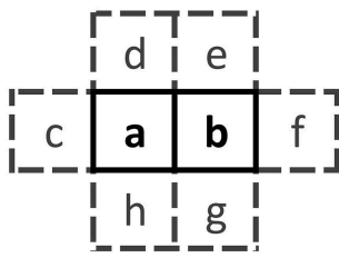
FIGURE 4 | Template for the neighborhood \chi consisting of the pair ab and its six nearest neighbors c through h . Each letter can take on the value 0 or 1.
