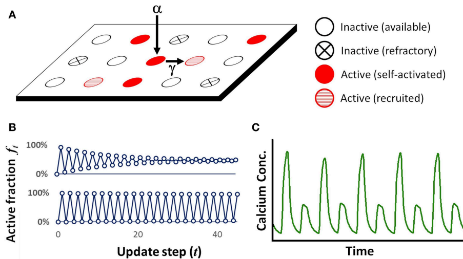
FIGURE 1 | (A) Illustration of lattice arrangement and possible states in the PCA. Available sites can self-activate with probability \alpha , or be recruited with probability \gamma . (B) Example of PCA lattice simulation showing the activation fraction f_t reaching either a steady state (top, for \gamma = 0.25 ) or maintaining periodicity (bottom, for \gamma = 0.75 ). In both cases \alpha was fixed at 0.80. (C) Simplified graphical representation of a typical experimental recording of calcium concentration over time in a cardiac myocyte, under conditions that produce alternans. Each peak represents either a high or low release of calcium, and peaks are \sim 150 – 300 ms apart.
